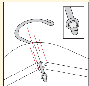
Punch In with Washer
